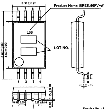
Fig4-(g) PHYSICAL DIMENSION SSOP-B8 (BR93L66FV-W)
